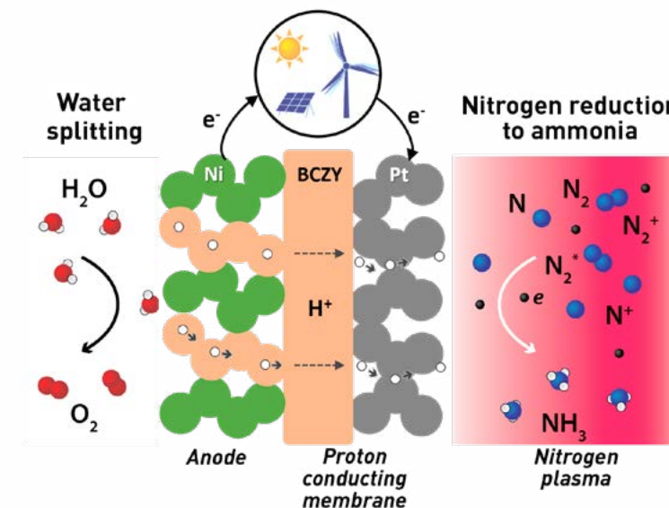
Ammonia production overview
