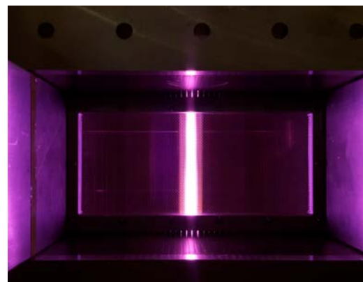
Argon plasma in newly built 6 kW labreactor
